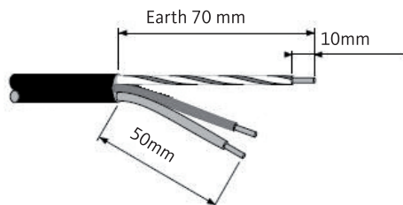
End of the power cable
