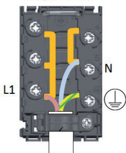
Factory connection
